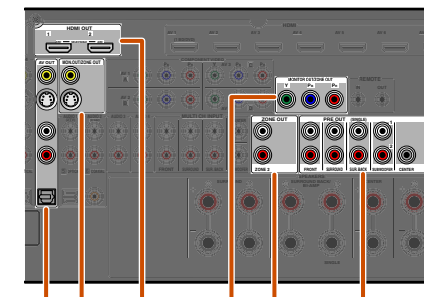
Output jacks
