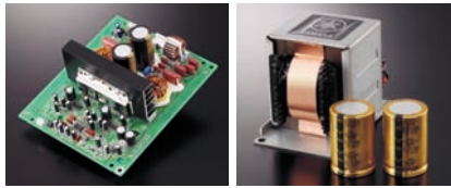
Yamaha original digital amplifier, and power transformer (4.2kg; 9.3lbs.) and custom-made block capacitors
